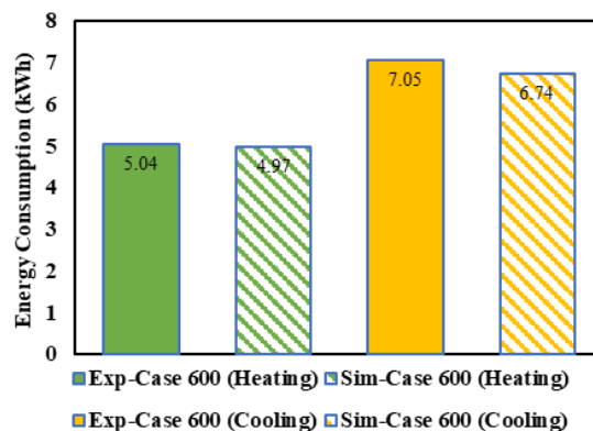
Figure 1. Comparison of the annual heating/cooling loads between ASHARE case 600 vs DesignBuilder simulations.
