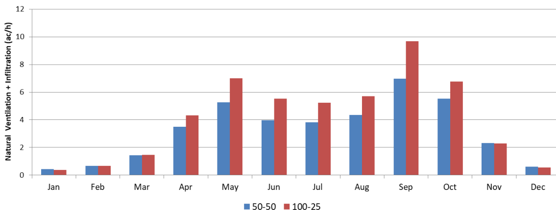
Figure 5. Air flow (ac/h) for the best (100-25) and the worst (50-50) models in providing natural ventilation.
