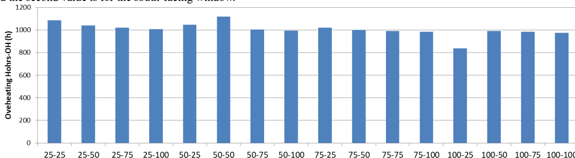
Figure 4. Overheating hours during the year for the case without DSF.
